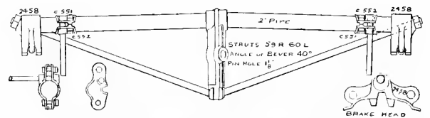
Figs. 1550-1552. Standard Outside Hung Freight Beam with Finger-Guards.
